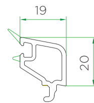
Double glazing bead-22mm VVI260-0060
