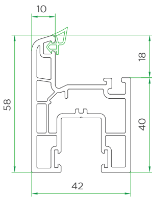
Sliding Sash VVI160-1040
