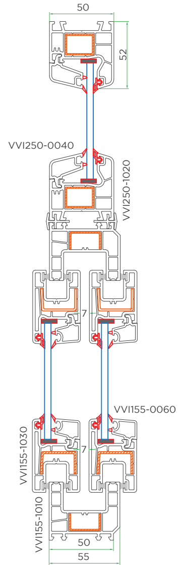
Cross sectional view-1
