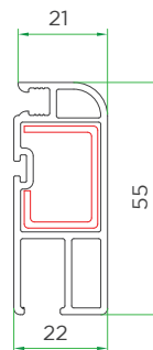
Mesh sash Rein 6001-1505
