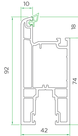
Sliding big door sash VVI160-1060
