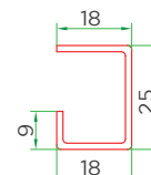
Mesh sash Rein 6001-1505
