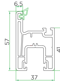
Sliding Sash VVI155-1030
