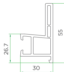
Add on Track VVI160-0130
