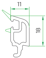
Double glazing bead (20mm) VVI250-0050
