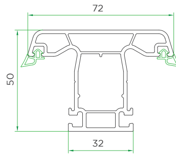
Casement Mullion VVI250-2030
