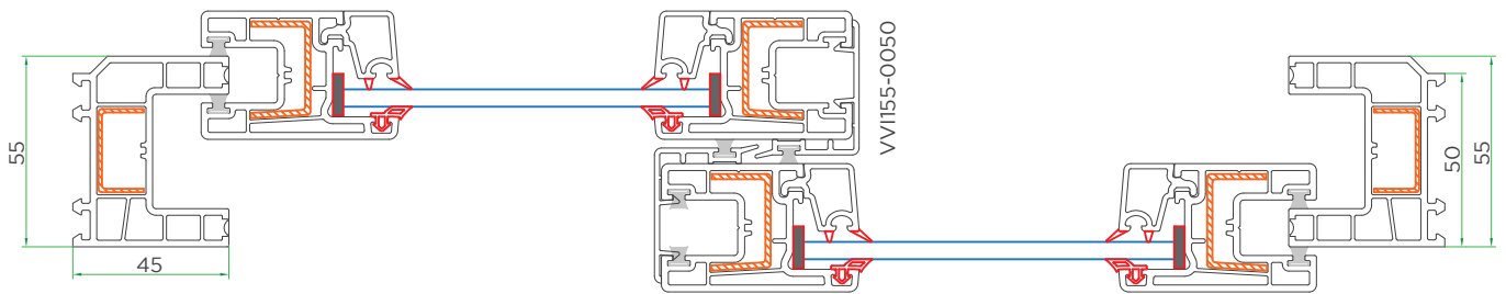
Cross sectional view-1
