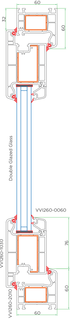
Cross sectional view-1
