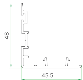
Sliding big door Sash Interlock VVI160-0100
