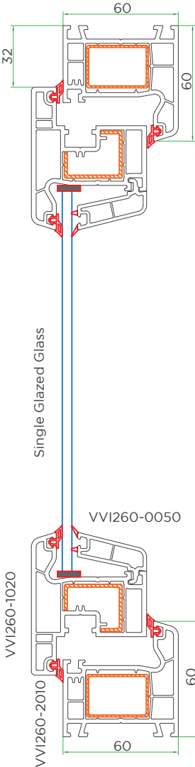
Cross sectional view-1
