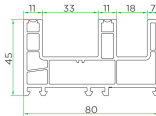
Sliding 2.5-track frame VVI155-1020
