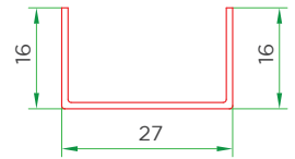
2.5-track Rein 6001-1002
