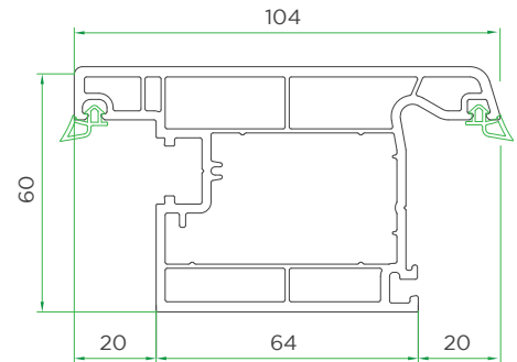
Casement Door Sash VVI260-1030
