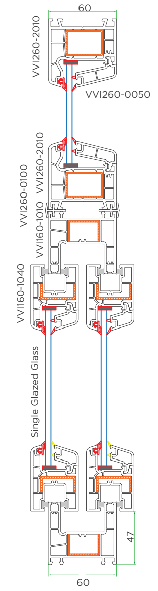
Cross sectional view-1
