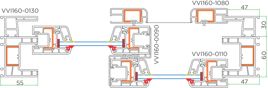
Cross sectional view-2
