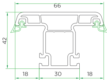
Sliding Mullion VVI160-1070
