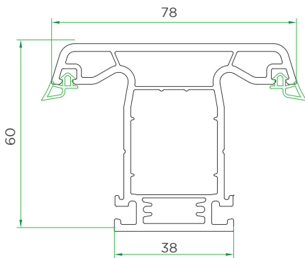
Casement Mullion VVI260-2040
