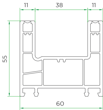
Sliding 2-track frame VVI160-1010
