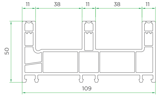
Sliding 3-track frame VVI160-1030
