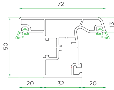
Casement Sash VVI250-1020
