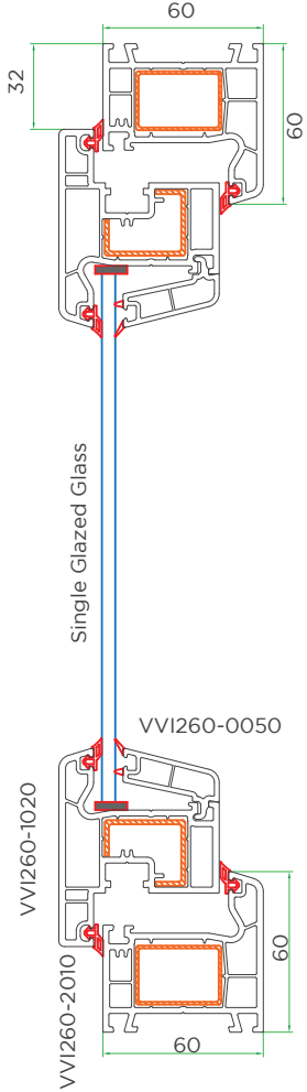
Cross sectional view-1
