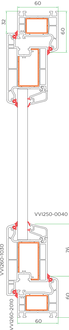
Cross sectional view-1
