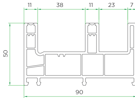
Sliding 2.5-track frame VVI160-1020
