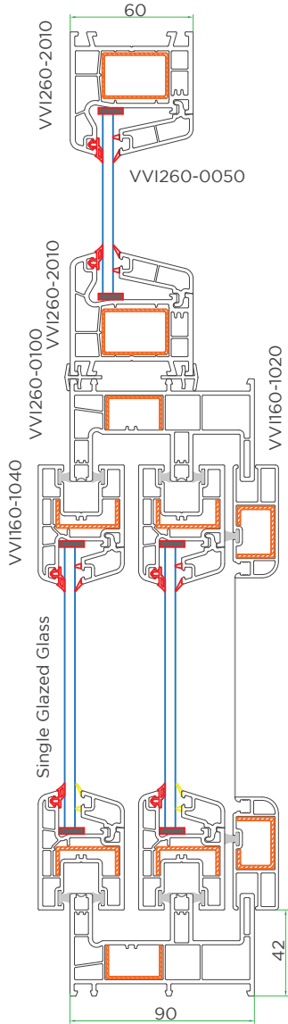
Cross sectional view-1
