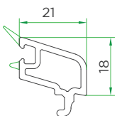
Single Glazing Bead(5mm) VVI160-0110
