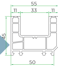
Sliding 2-track frame VVI155-1010
