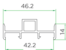
Sliding Sash Connector VVI160-0120
