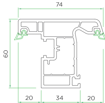
Casement Window Sash VVI260-1020
