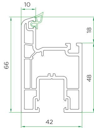
Sliding door sash VVI160-1050
