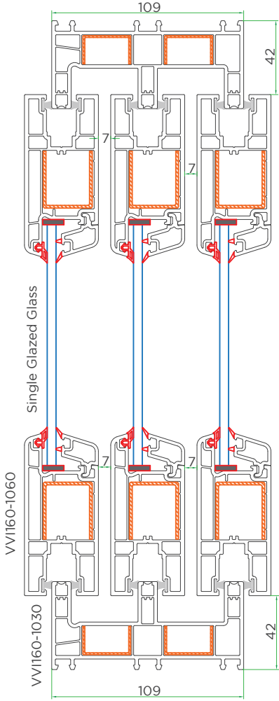
Cross sectional view-1
