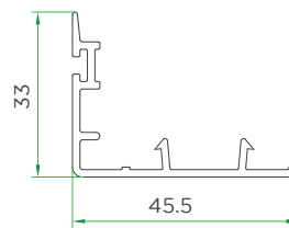
Sliding Sash Interlock VVI160-0090
