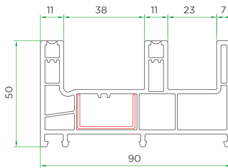
2-track Rein 6001-1001
