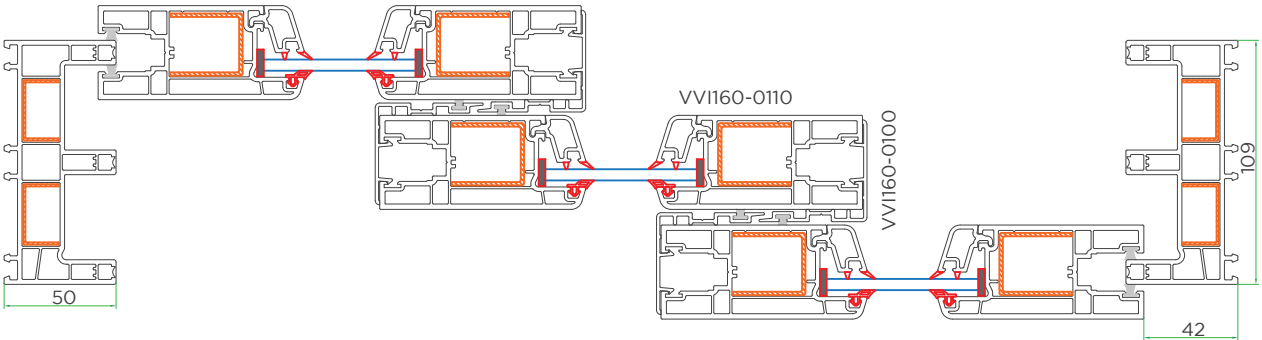
Cross sectional view-2
