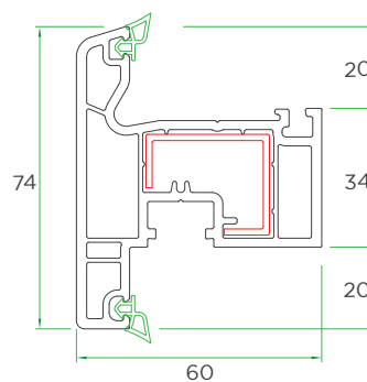
Frame Rein 6002-1001
