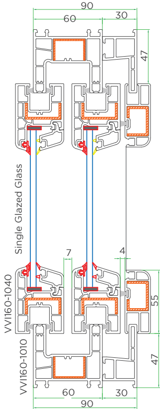
Cross sectional view-1
