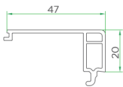
Louver Bead VVI260-0070
