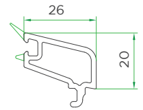
Single glazing bead (5mm) VVI250-0040
