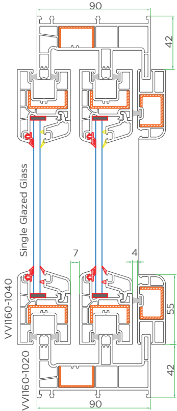
Cross sectional view-1
