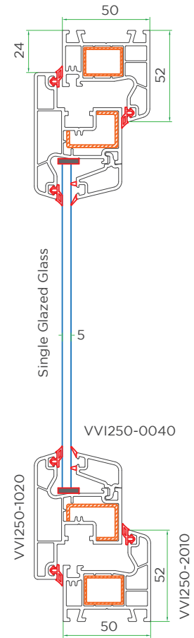
Cross sectional view-1
