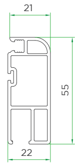
Mesh Sash profile VVI160-1080
